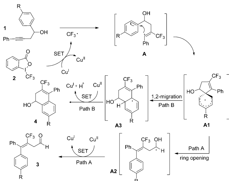
Scheme 3. Proposed mechanism.
